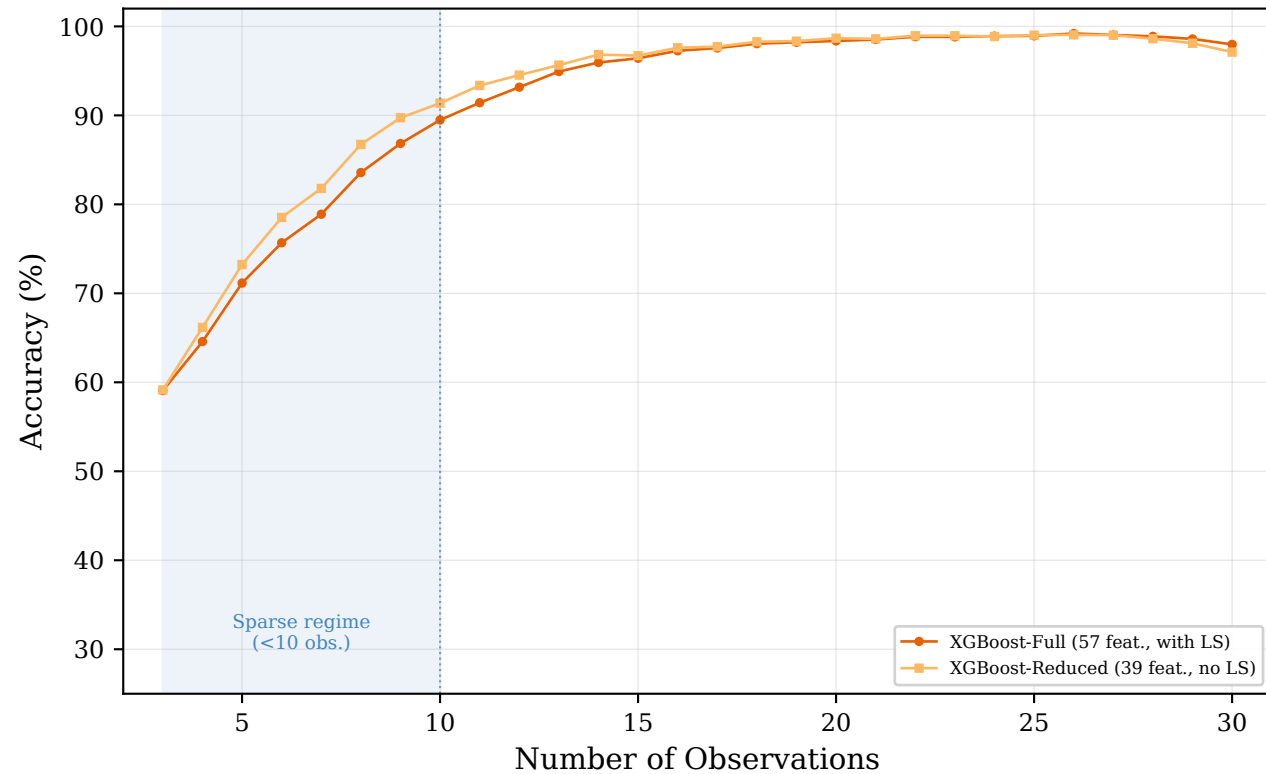
(a) XGBoost-Full vs. XGBoost-Reduced
